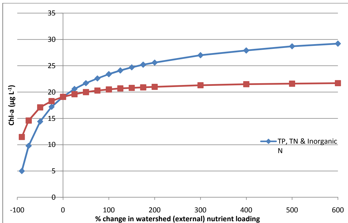
Figure 17 Lake Hefner Chl- a Response to % Changes in Watershed Nutrient Loads. Red squares = change in TP load only, blue diamonds = change in TP, TN and inorganic N loads
