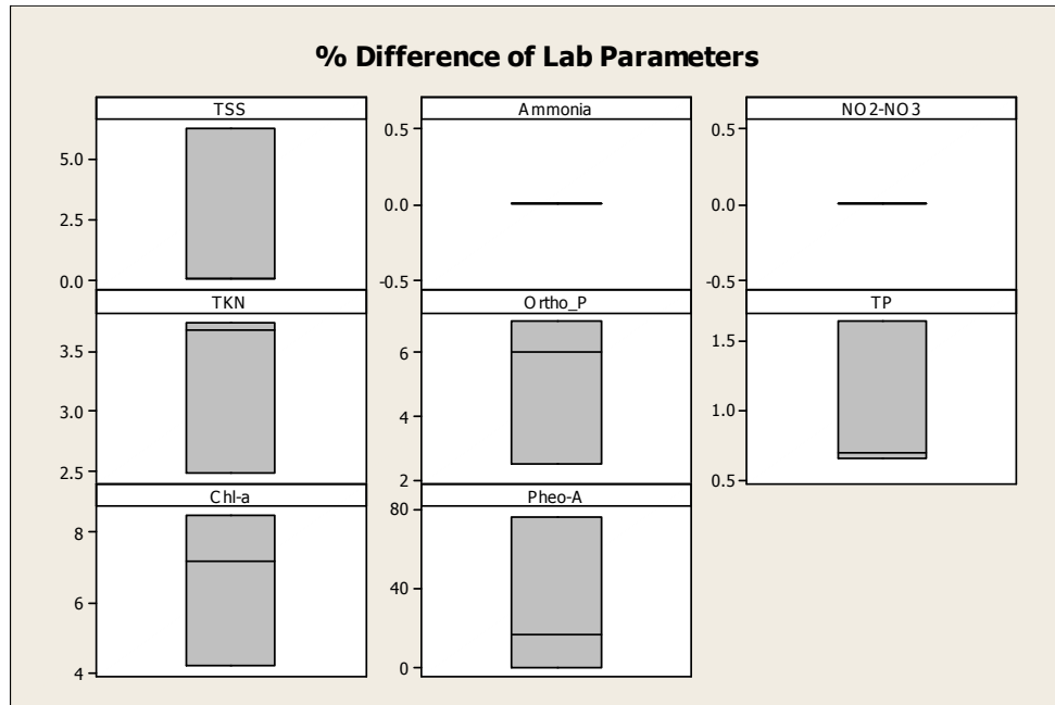
Figure 4 Percent Difference of Total Suspended Solids (TSS), Ammonia, Nitrate-nitrite (NO2-NO3), total Kjeldahl nitrogen (TKN), Ortho-phosphate (Ortho-p), total phosphorous (TP), chlorophyll-a (Chl-a), and pheophytin-a (Pheo-a).
