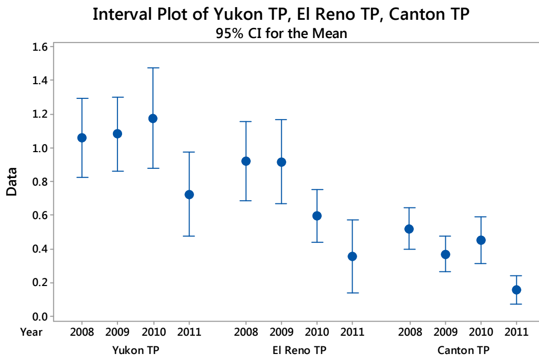
Figure 13 Interval Plot of North Canadian River Mean TP Concentrations (mg L -1 ) at Yukon, El Reno and below Canton Lake.
