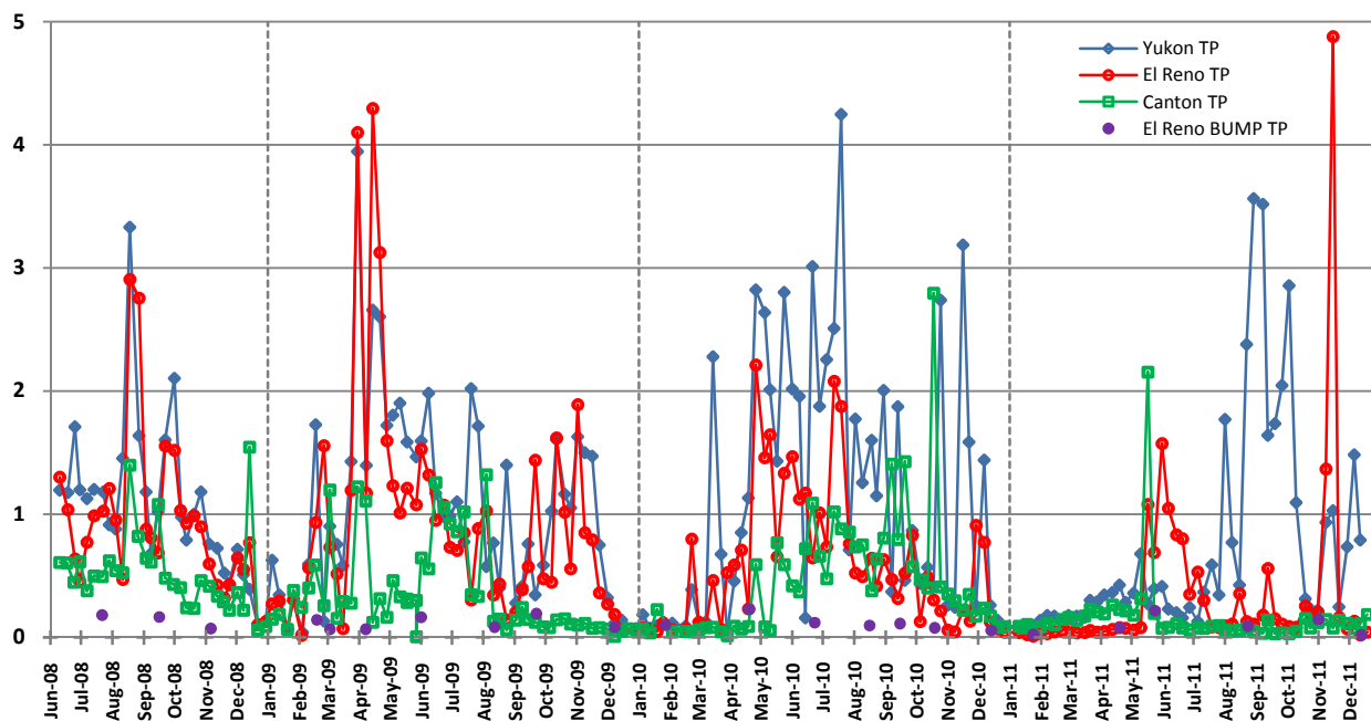
Figure 11 North Canadian River Total Phosphorus Concentrations ( \text{mg L}^{-1} ) at Yukon (hollow diamonds), El Reno (hollow circles = OCC data; solid circles= BUMP data) and Canton Lake (hollow squares).
