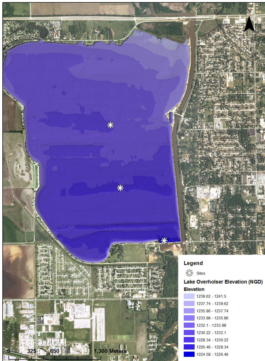
Figure 3 Lake Overholser sample sites
