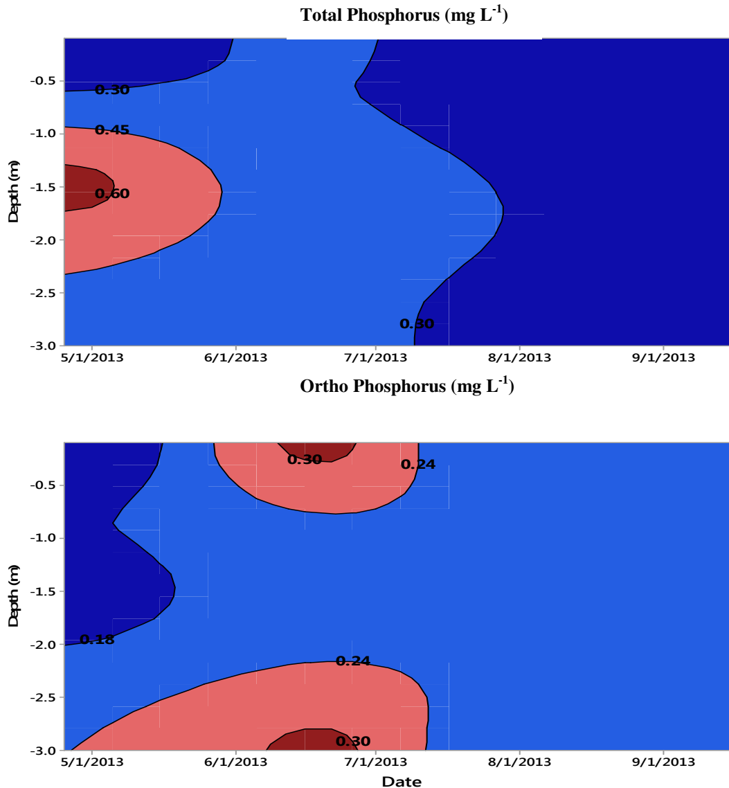
Figure 10 Lake Overholser Isopleths Plots Showing Total Phosphorus (mg L -1 ) and Ortho-phosphorus (mg L -1 ). Note that due to the shallow depth of Lake Overholser these isopleths are based on limited vertical measurements (0.5, 1.5 and 3 m) and due to analysis constraints the 1.5 m depth was only sampled at site 1 once during 2013.
