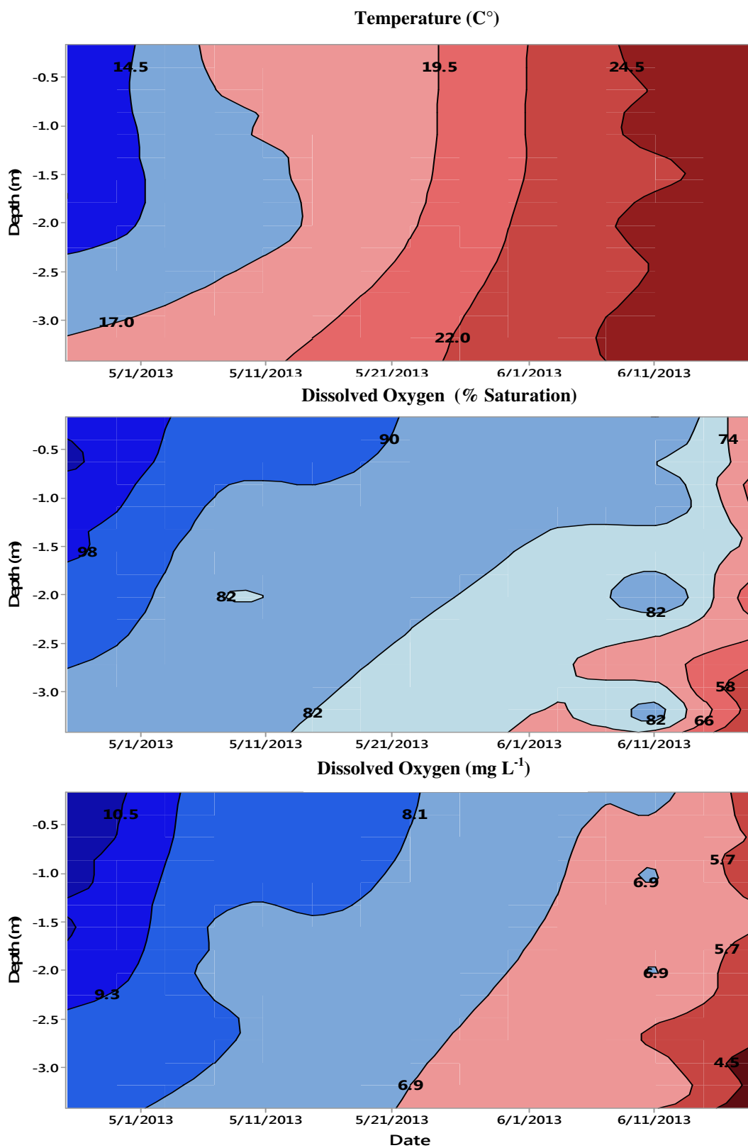
Figure 8 Lake Overholser Isopleths Plots Showing Temperature (C°), Dissolved Oxygen (% Saturation), and Dissolved Oxygen (mg L -1 ).
