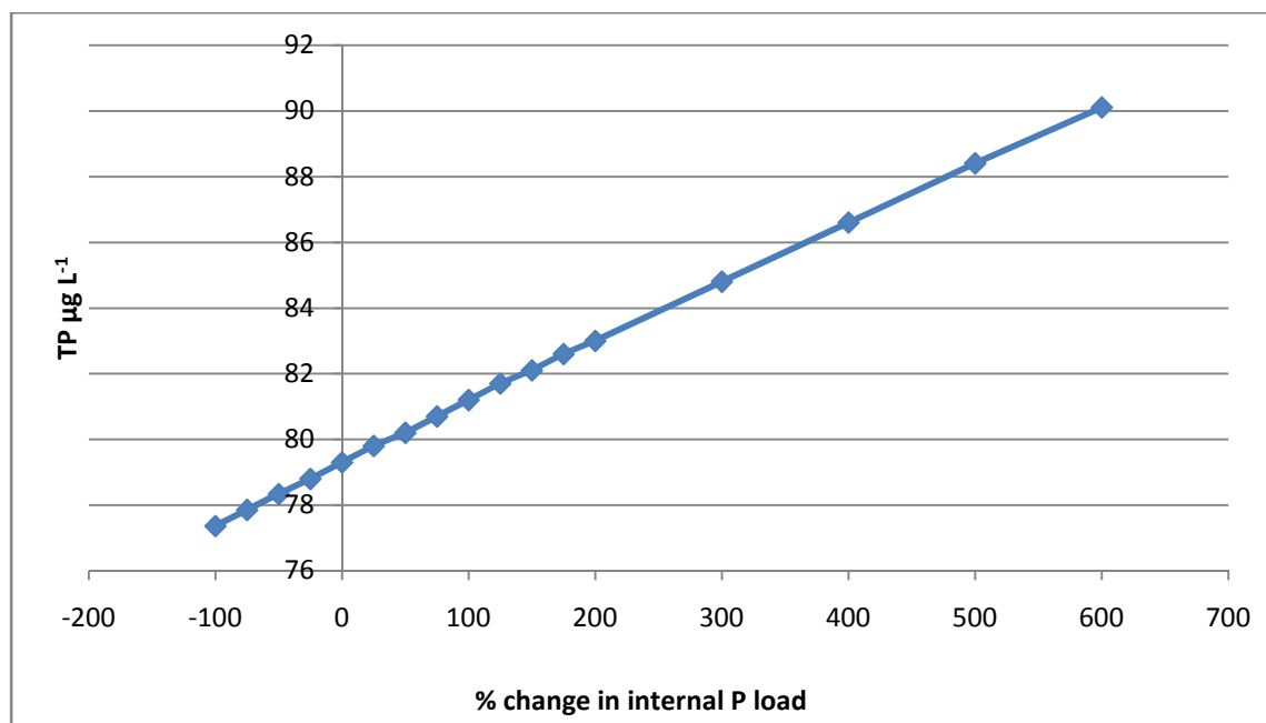
Figure 16 Lake Hefner % Change in Internal P Load and Effect of Lake TP Concentrations ( \mu\text{g L}^{-1} ).
