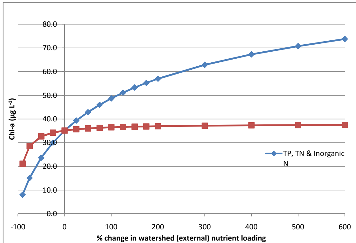
Figure 18 Lake Overholser Chl-a Response to % Changes in Watershed Nutrient Loads. Red squares = change in TP load only, blue diamonds = change in TP, TN and inorganic N loads
