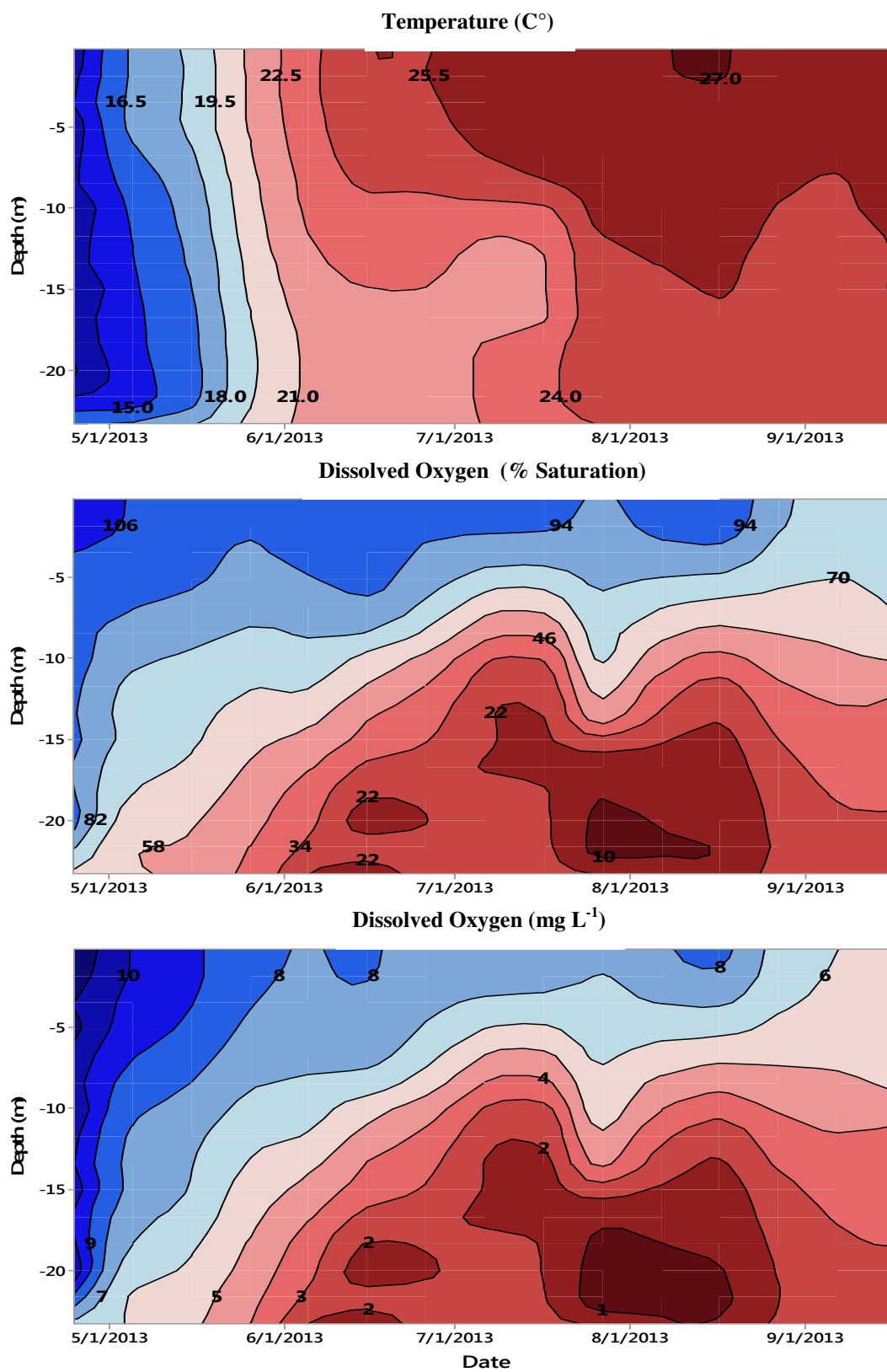
Figure 7 Lake Hefner Isopleths Plots Showing Temperature (C°), Dissolved Oxygen (% Saturation) & Dissolved Oxygen (mg L -1 ).
