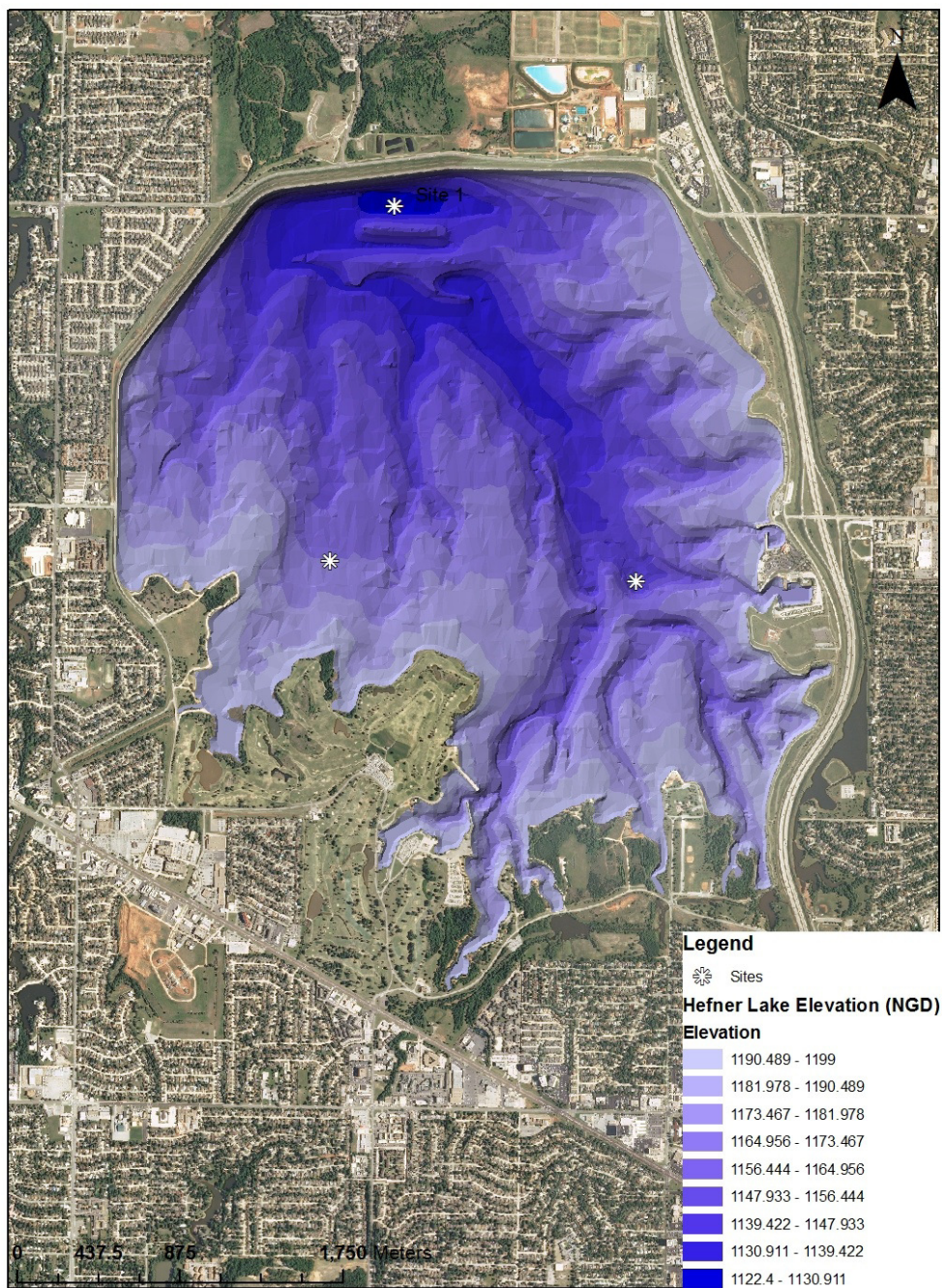
Figure 2 Lake Hefner sample sites.
