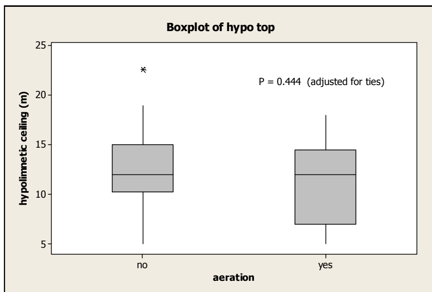
Figure 6 Box Plot of Depth to the Top of the Hypolimnion During Periods of 'No' Aeration (post-1995) and 'Yes' Aeration (post-1995) for Lake Hefner.
