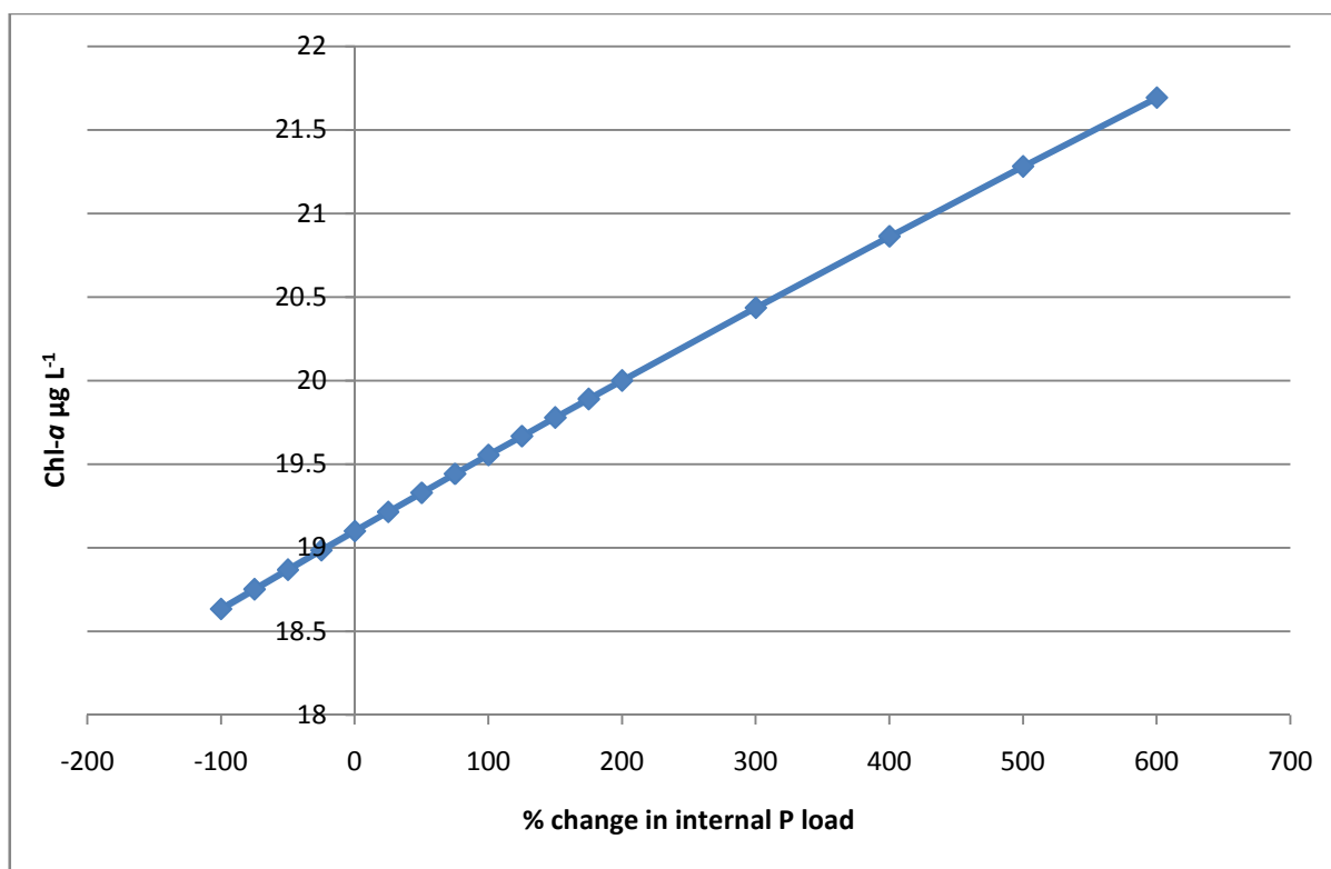
Figure 15 Lake Hefner % Change in Internal P Load and Effect on Lake Chl-a Concentrations ( \mu\text{g L}^{-1} ).
