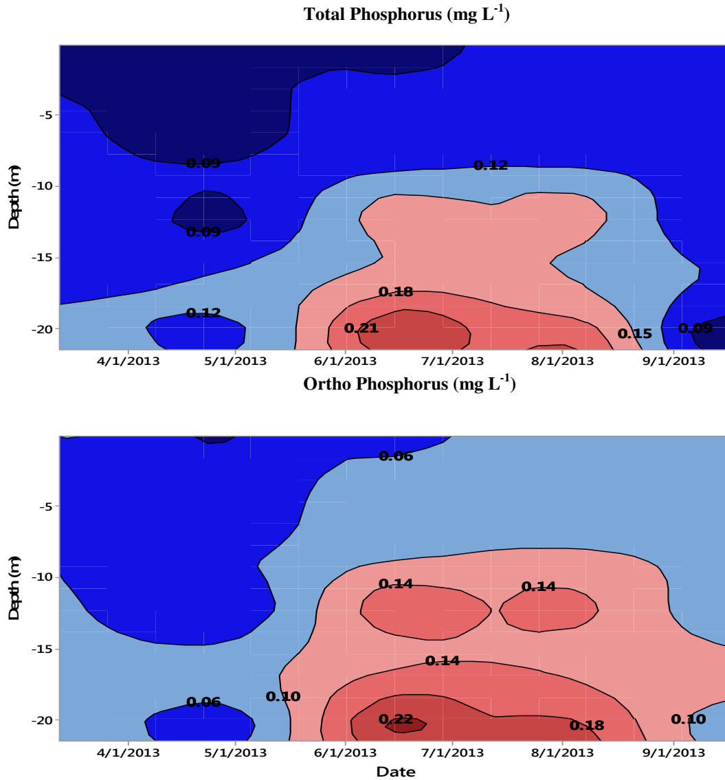
Figure 9 Lake Hefner Isopleths Plots Showing Total Phosphorus ( \text{mg L}^{-1} ) and Ortho-phosphorus ( \text{mg L}^{-1} ).
