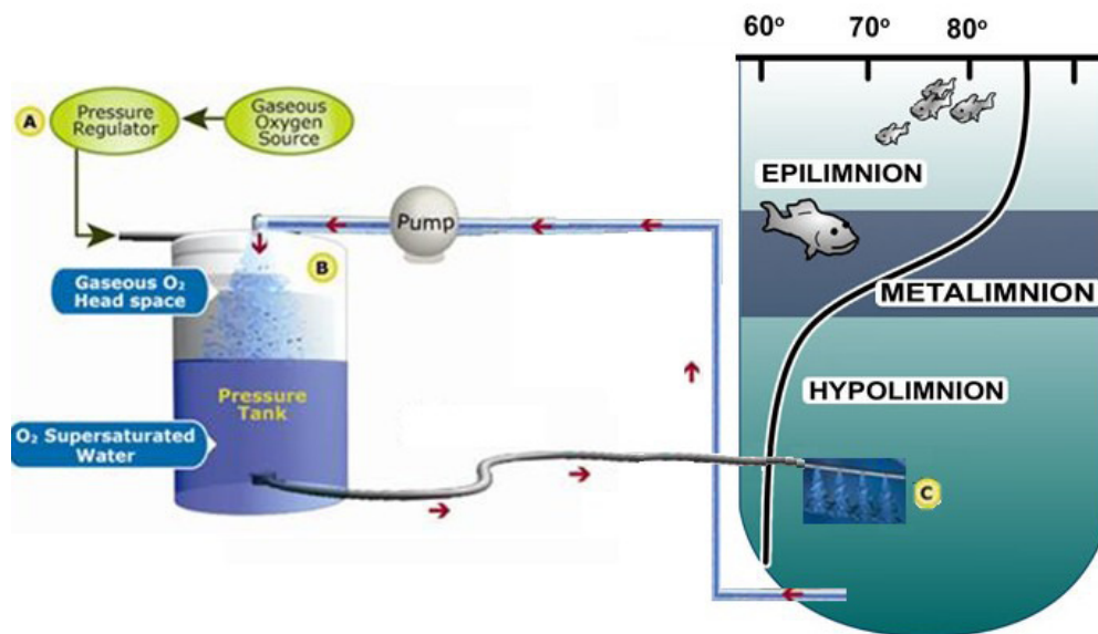
Figure 14 Conceptual Illustration of the SDOX System at Lake Thunderbird.
