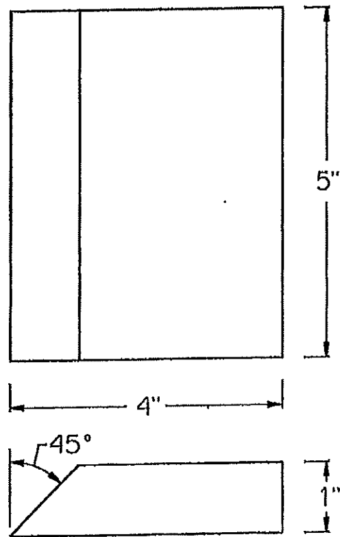
PLATE 4-1 (2G TEST)
