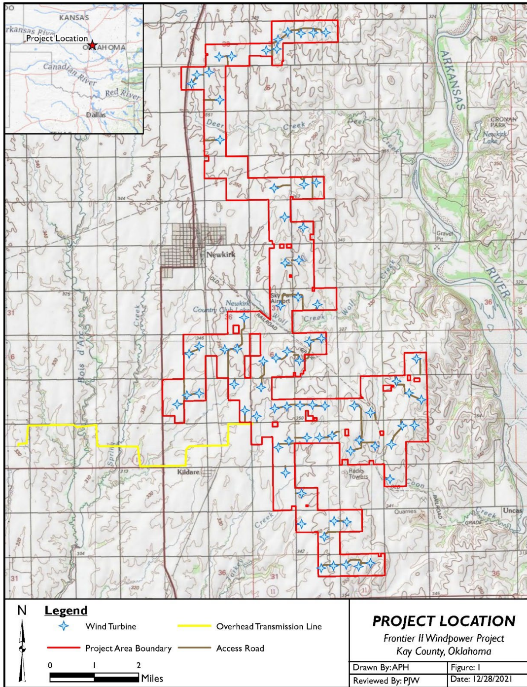
Figure 1. Location and Layout of the Frontier II Windpower Project
