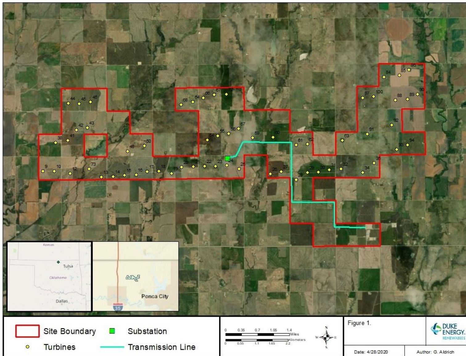
Figure 1. Location and Layout of the Frontier Windpower Project
